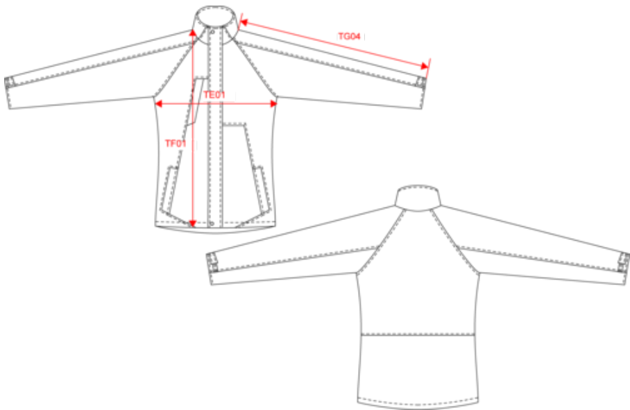
Dimensions (cm)
